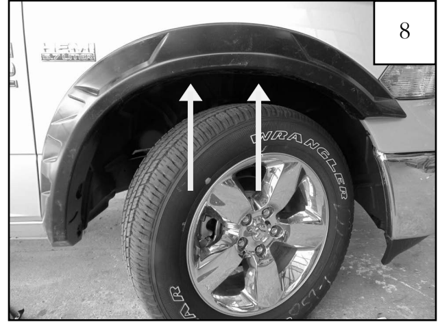
Hold flare to vehicle and start the supplied screws (SW1-0056) with a Phillips screwdriver. Do not tighten.
