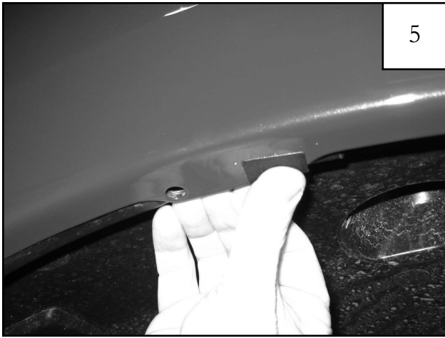
Install Tab (MT1-0014) over existing factory hole. There are two holes at the top center location. Refer to step 4 for proper hole for installation.
